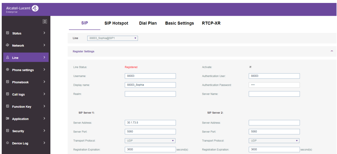
Figure 11 - SIP registration in web
