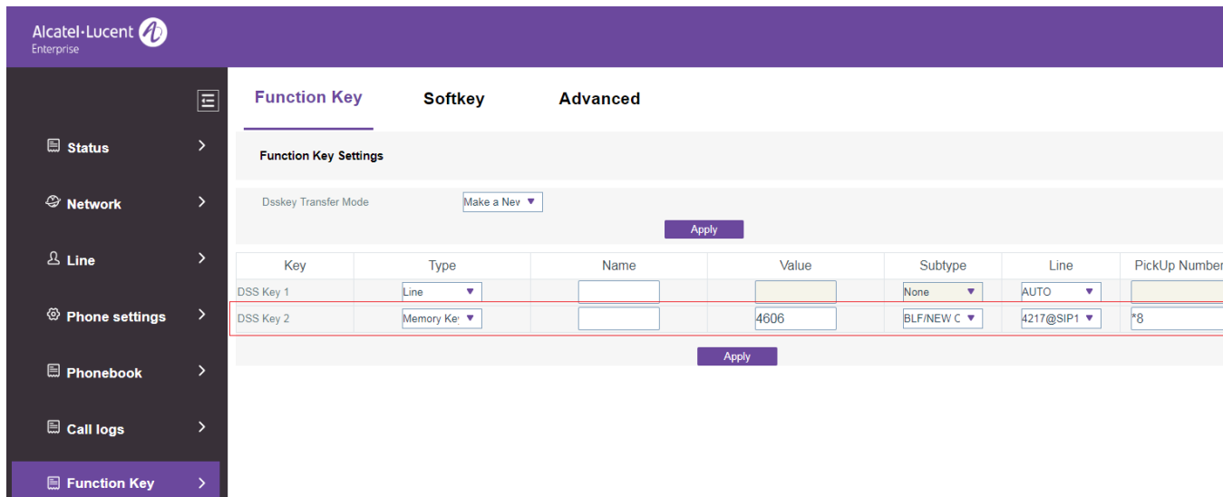
Figure 46 - Setting Pick Up on the web
