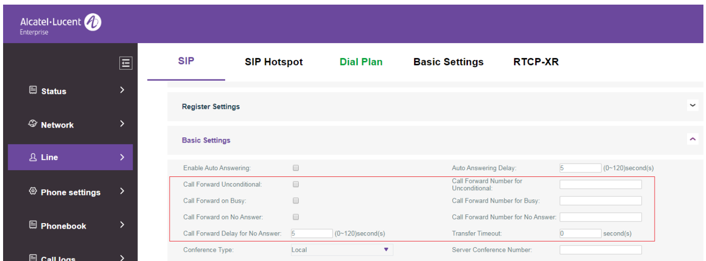
Figure 33 - Set call forwarding
