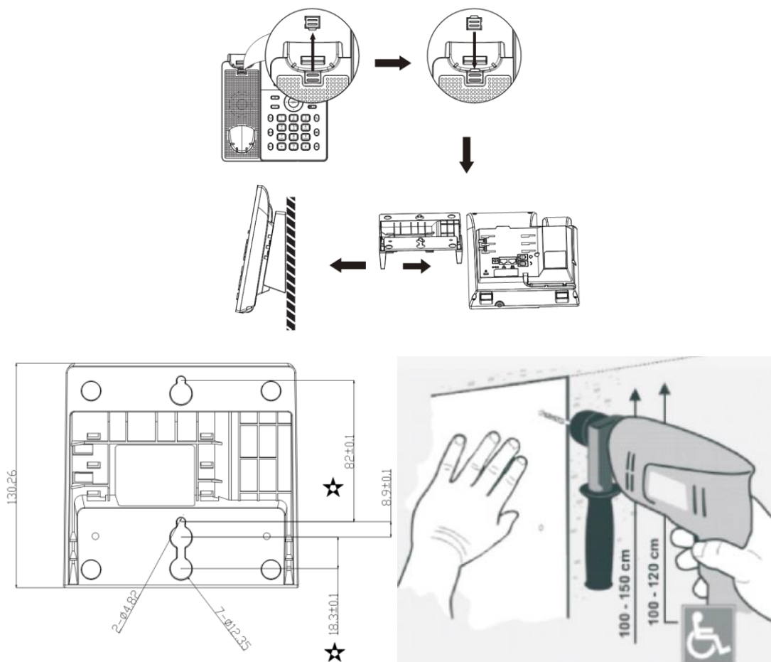
Figure 2 - Wall-mounted installation
