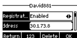
Figure 99 - SIP address and account information
