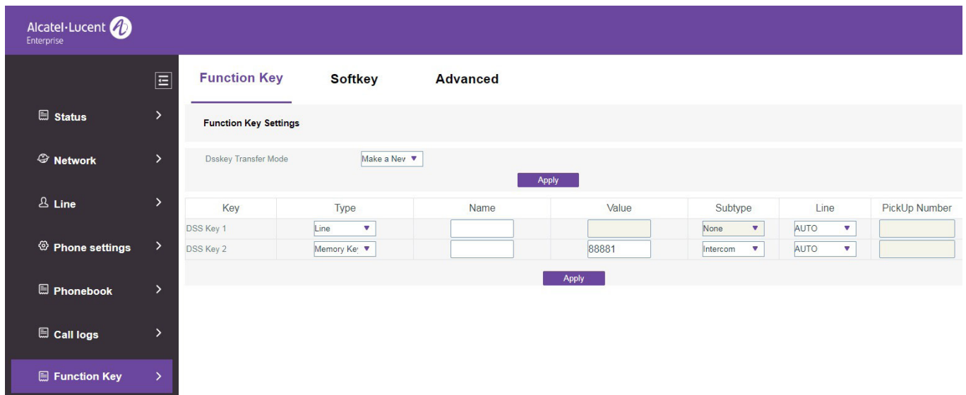
Figure 65 - Configuring the Intercom key on the web
