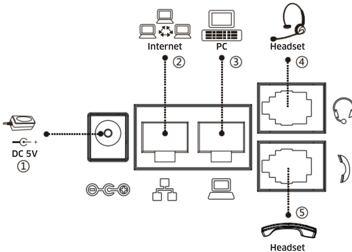
Figure 3 - Connecting to the device
