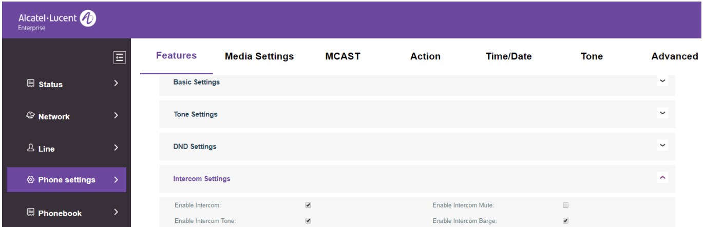
Figure 64 - Configuring the intercom on the Web
