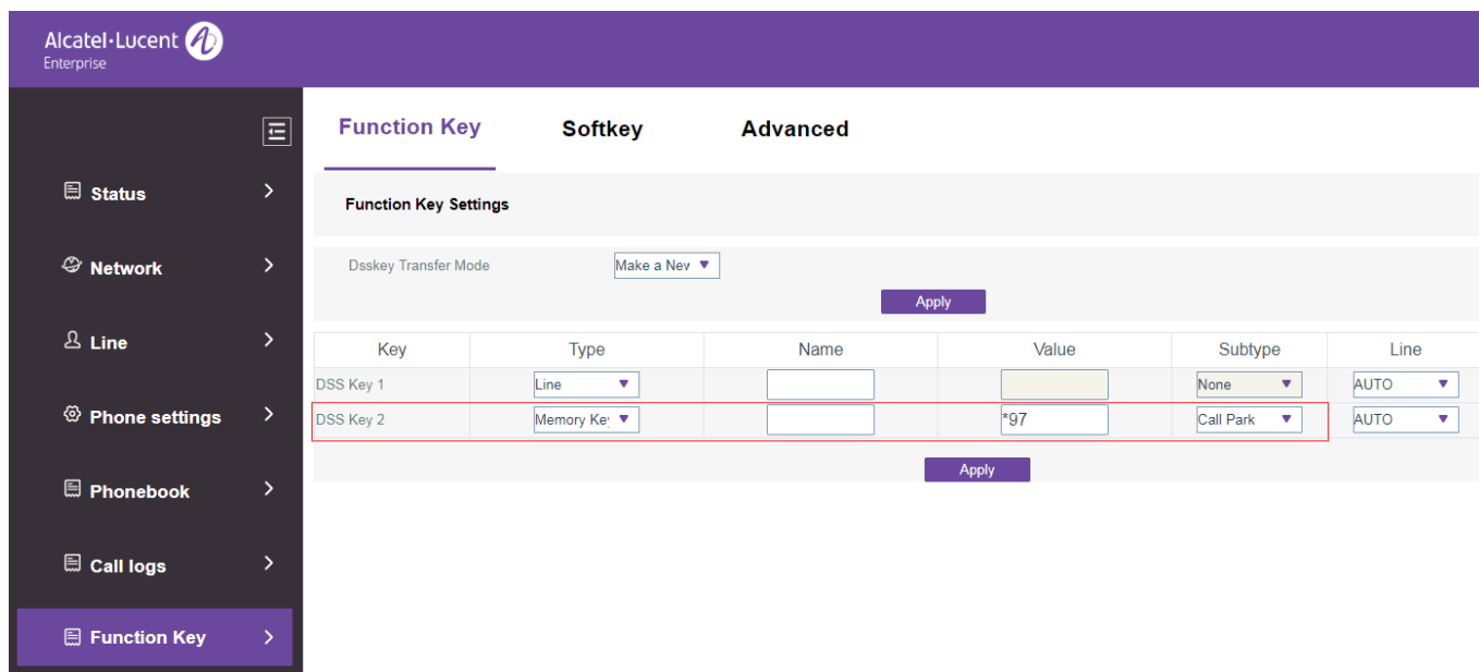
Figure 44 - Setting Call Park in web
